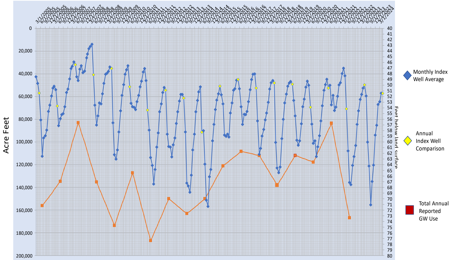
COASTAL BEND GROUNDWATER CONSERVATION DISTRICT INDEX WELL GRAPH - May 1, 2024
