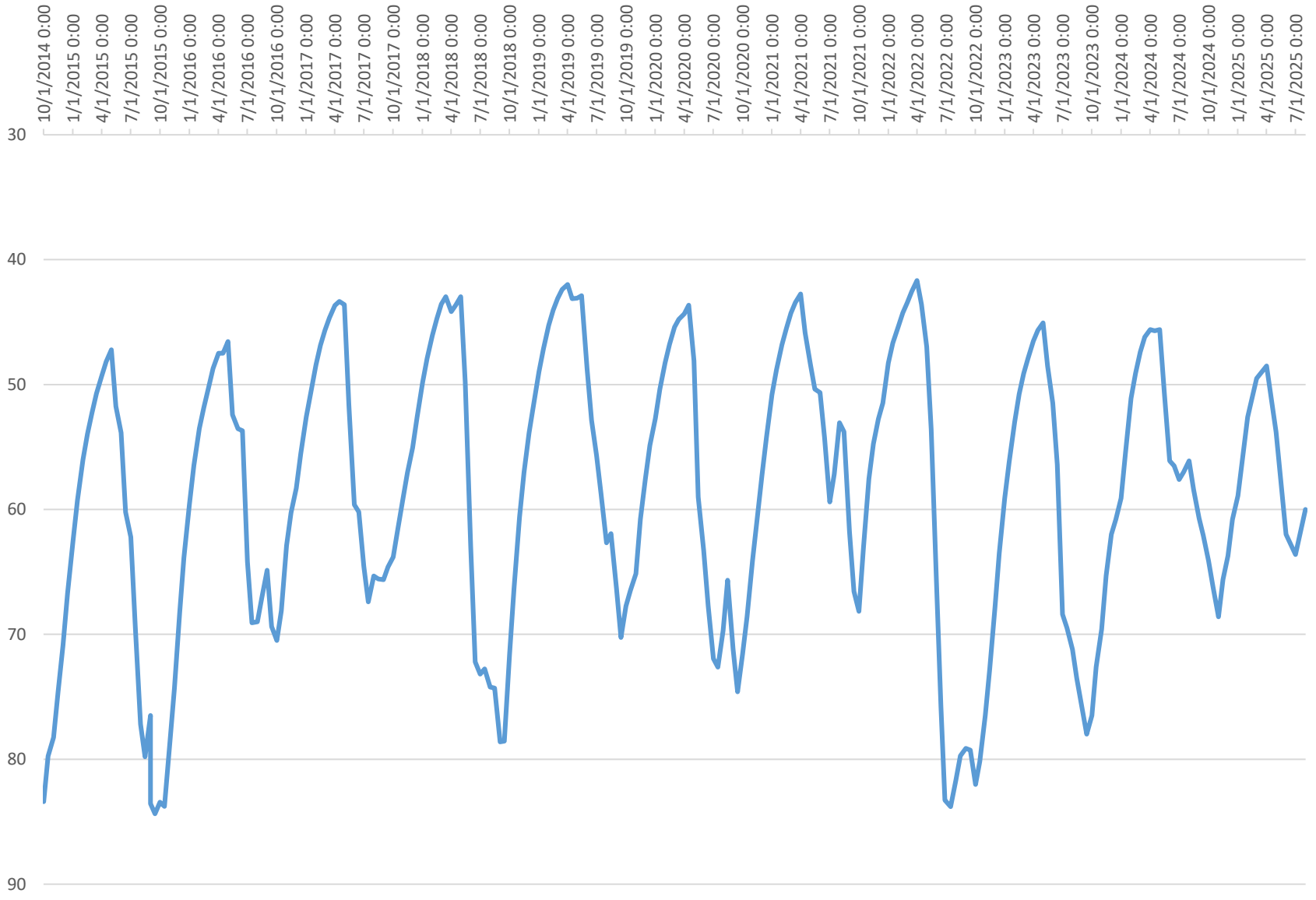
Lissie, TX Transducer - Depth to Water (ft) August 1, 2025
